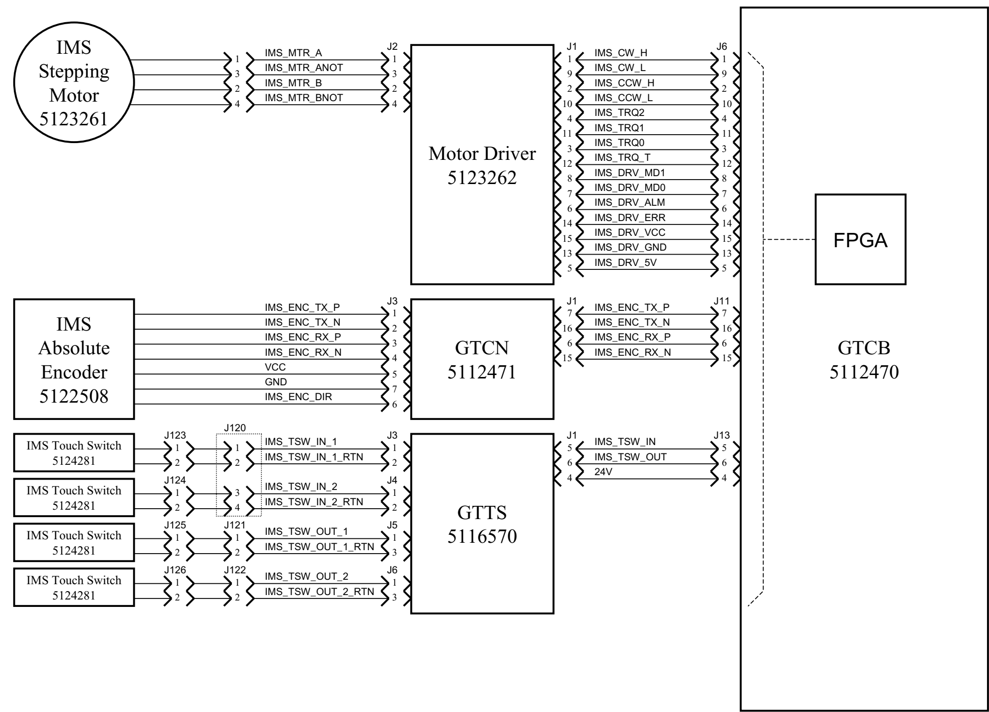
Figure 4-5 5127766 Sheet 2, Rev. 1
