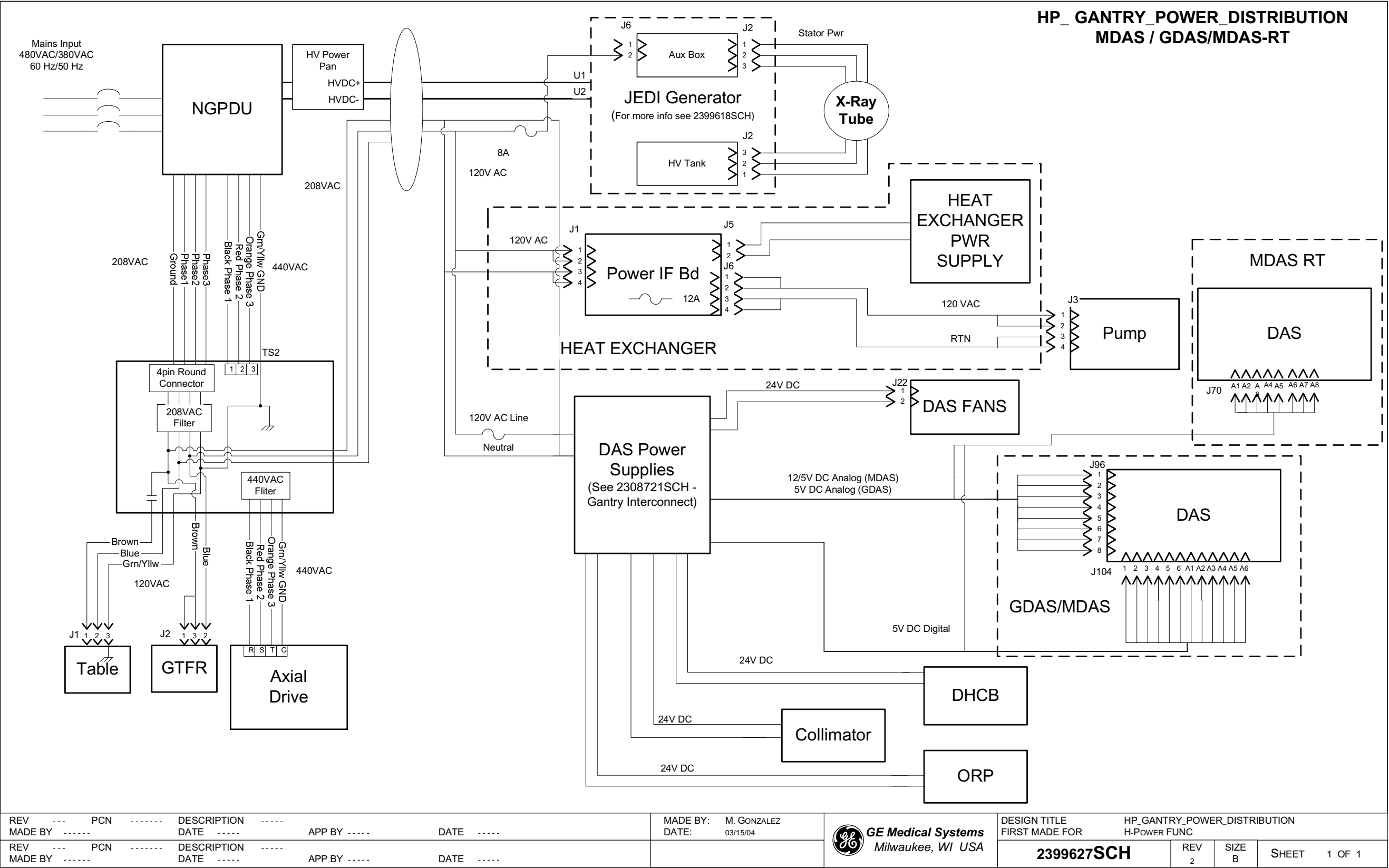
Figure 8-4 2399627 Sheet 1, Rev. 2
