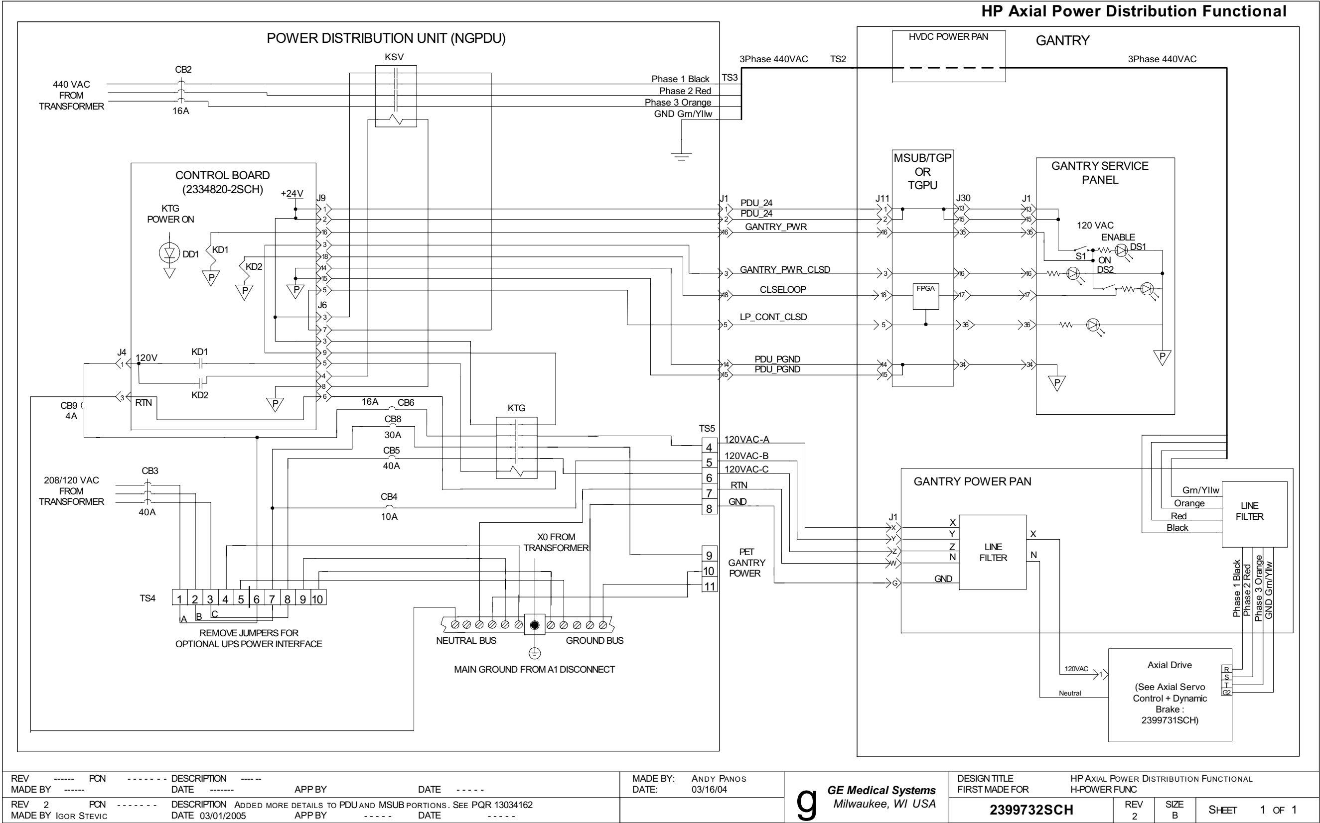
Figure 5-2 2399732 Sheet 1 Rev. 2
