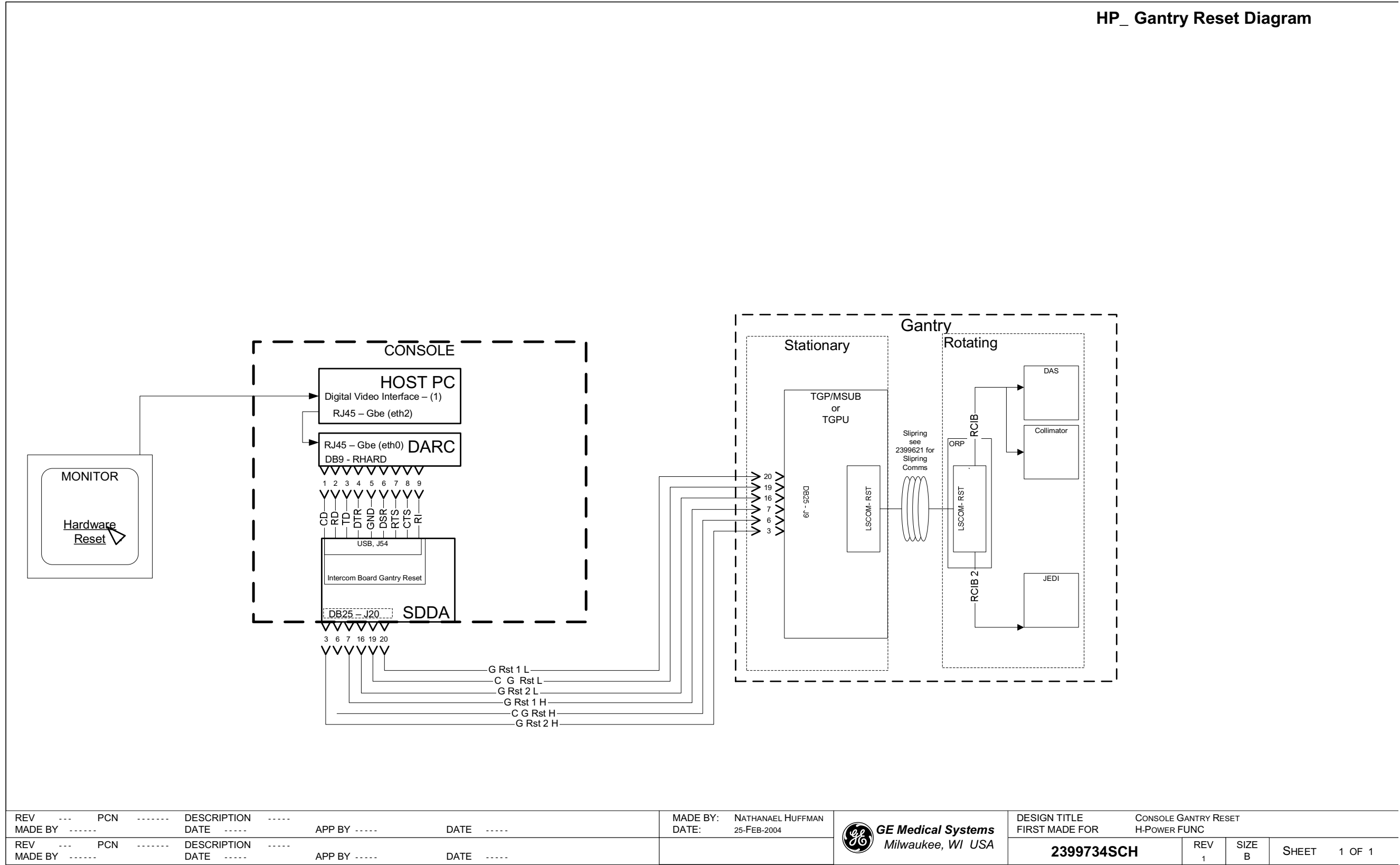
Figure 6-2 2399734 Sheet 1, Rev. 1
