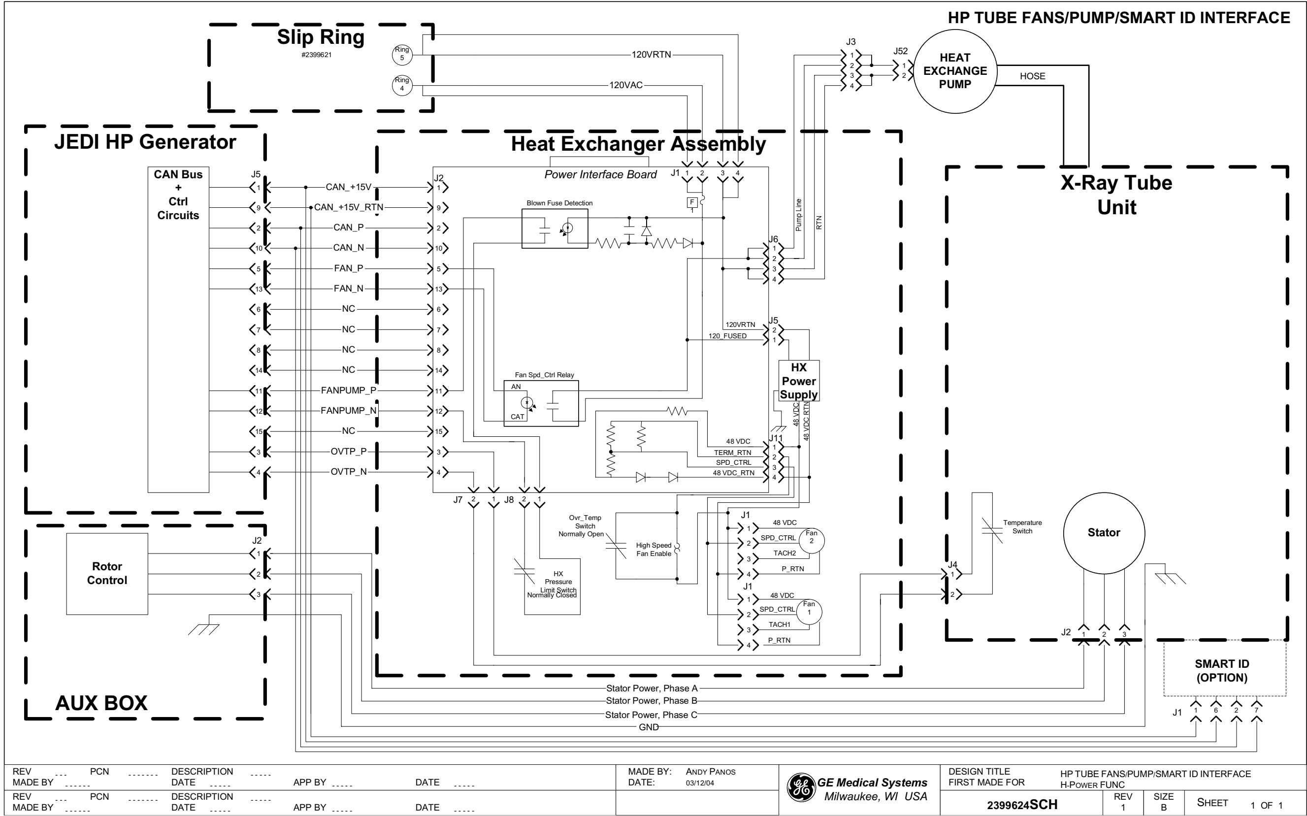
Figure 2-1 2399624 Sheet 1, Rev. 1
