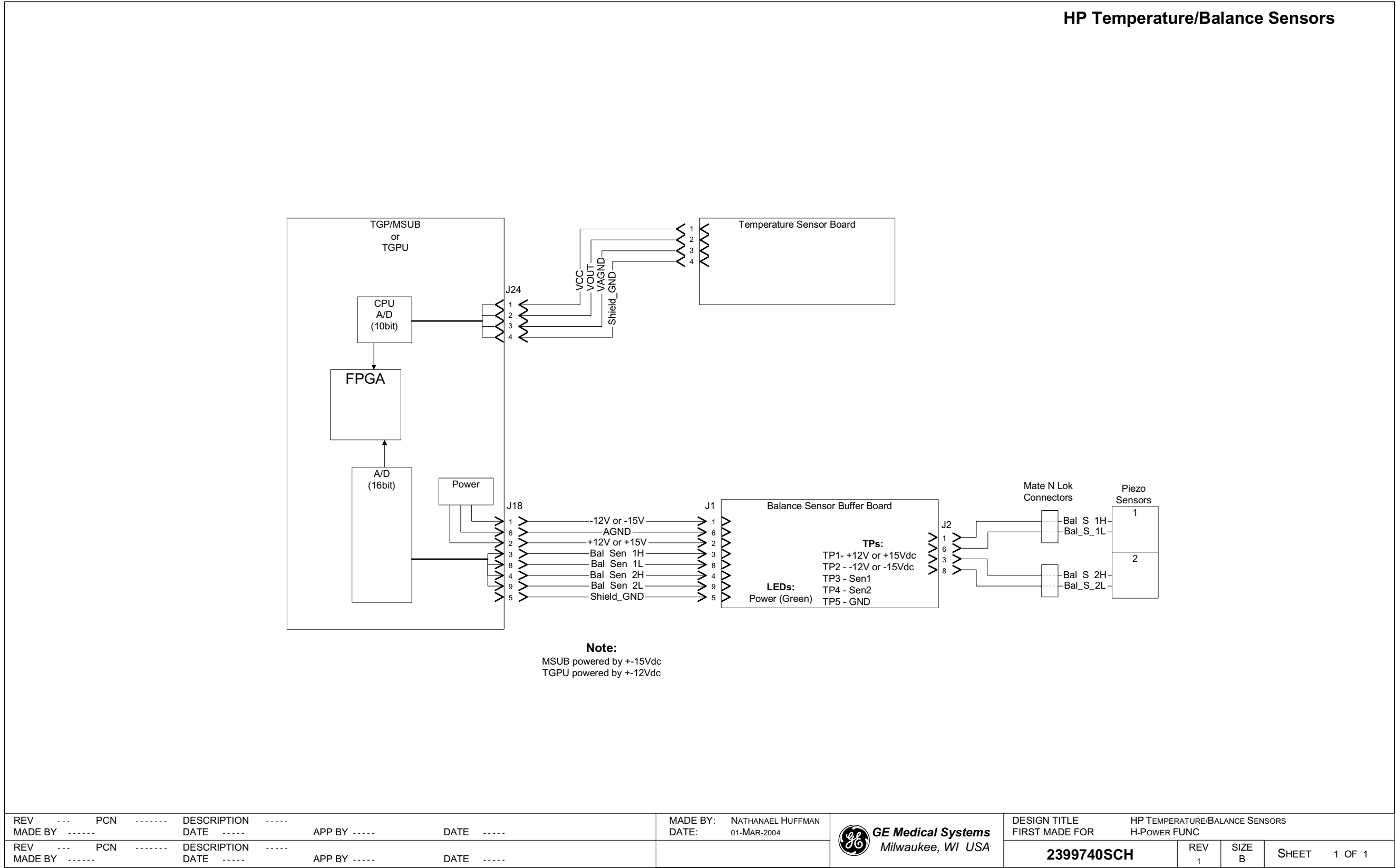
Figure 7-1 2399740 Sheet 1, Rev. 1
