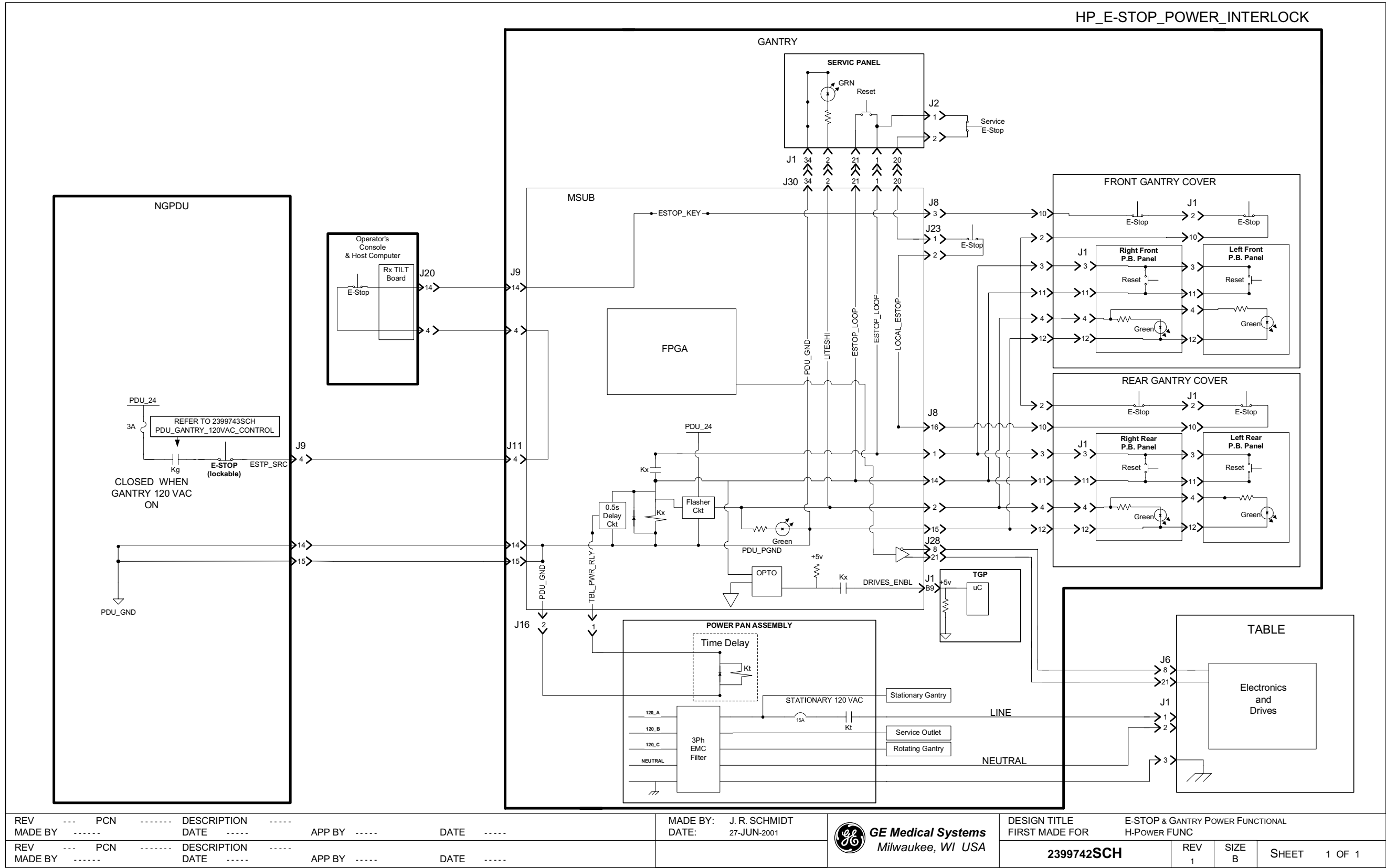
Figure 8-1 2399742 Sheet 1, Rev. 1
