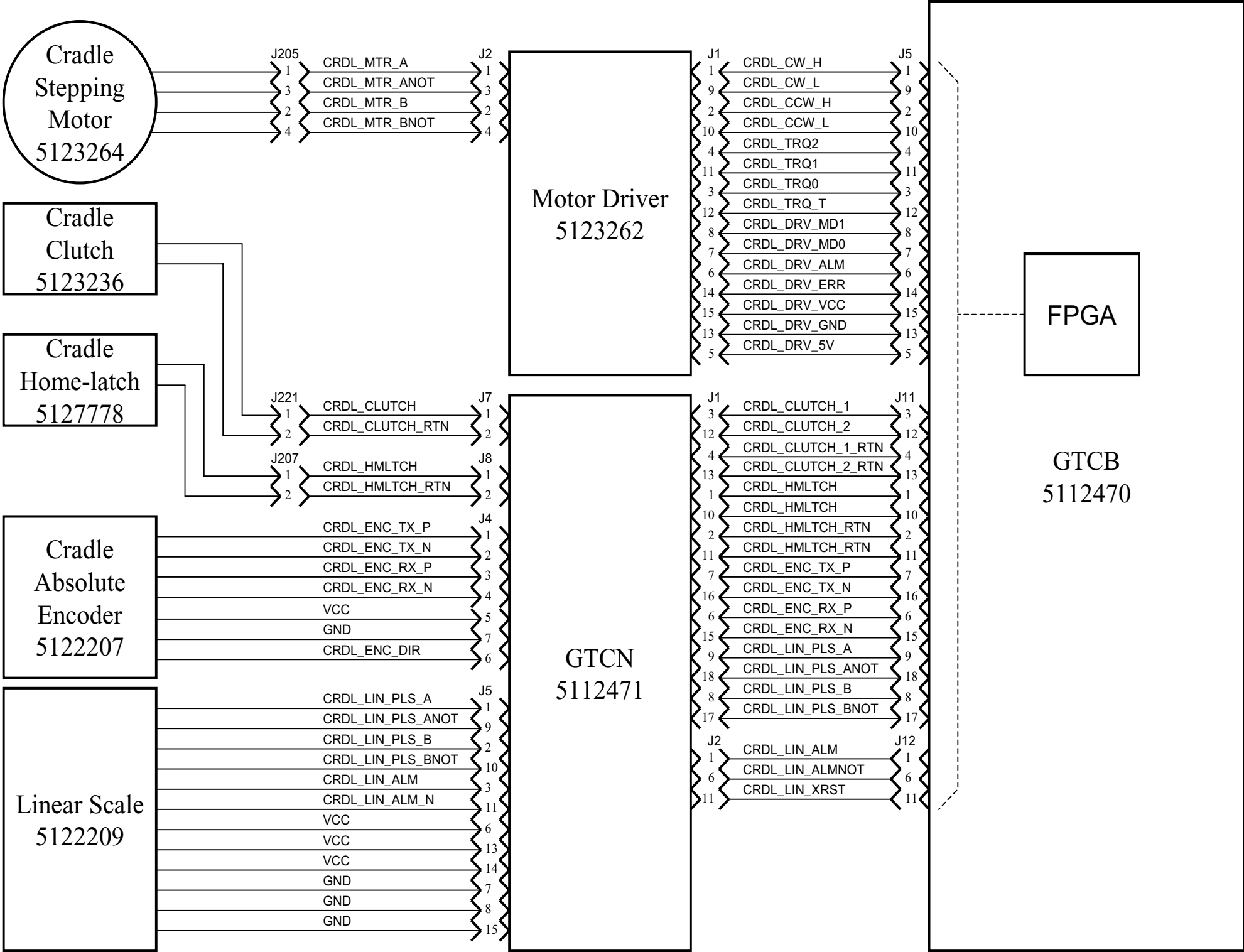
Figure 4-4 5127766 Sheet 1, Rev. 1
