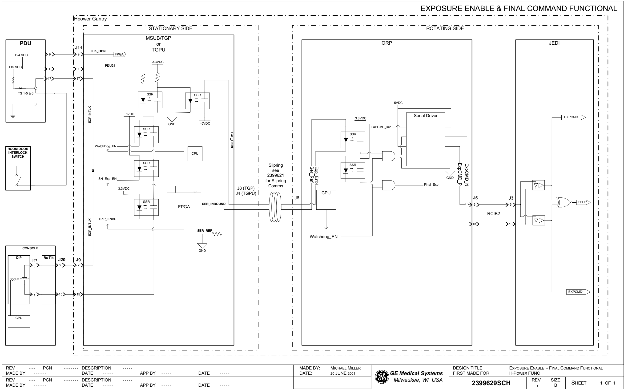
Figure 2-5 2399629 Sheet 1, Rev. 1
