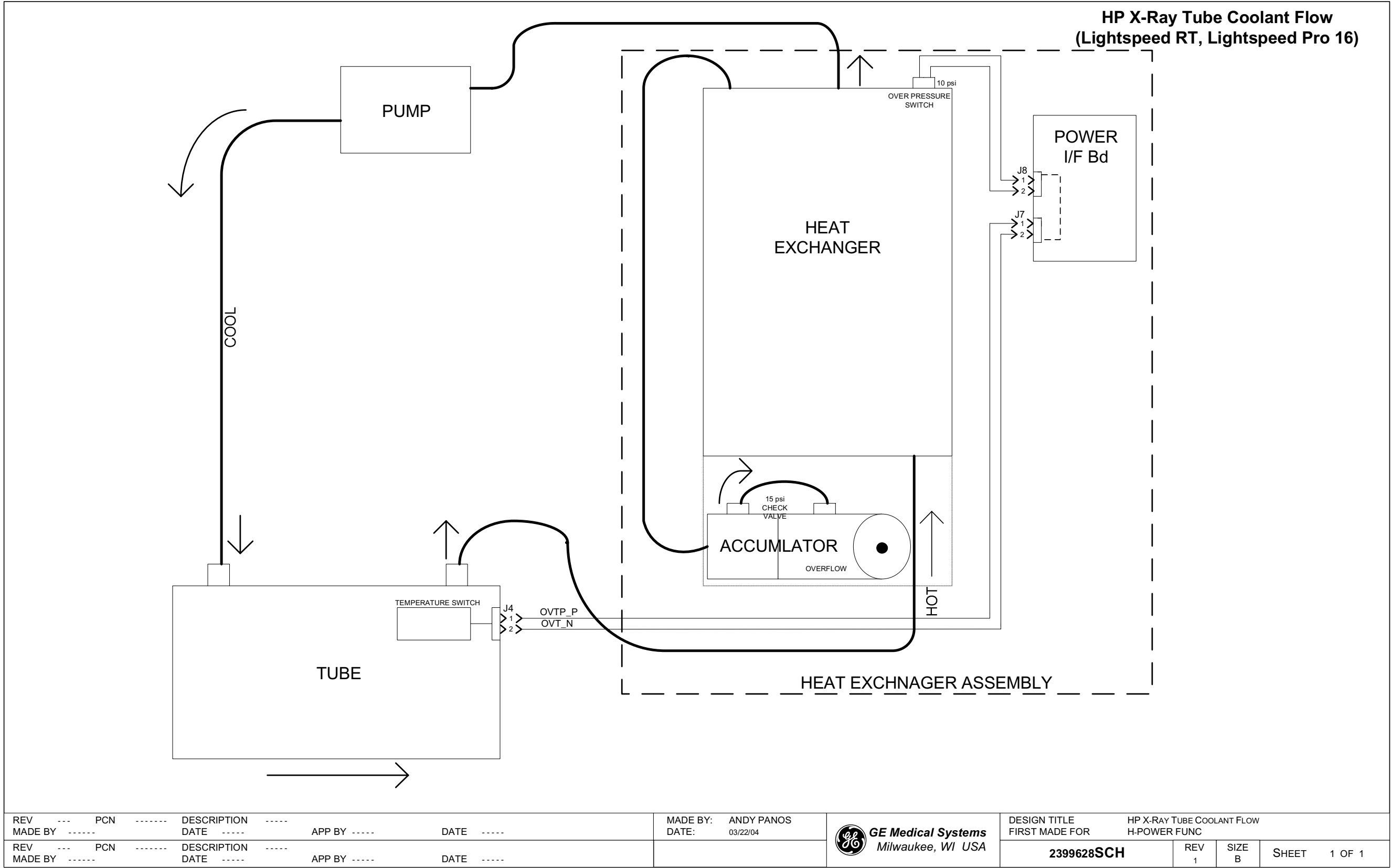
Figure 2-7 2399628 Sheet 1, Rev. 1
