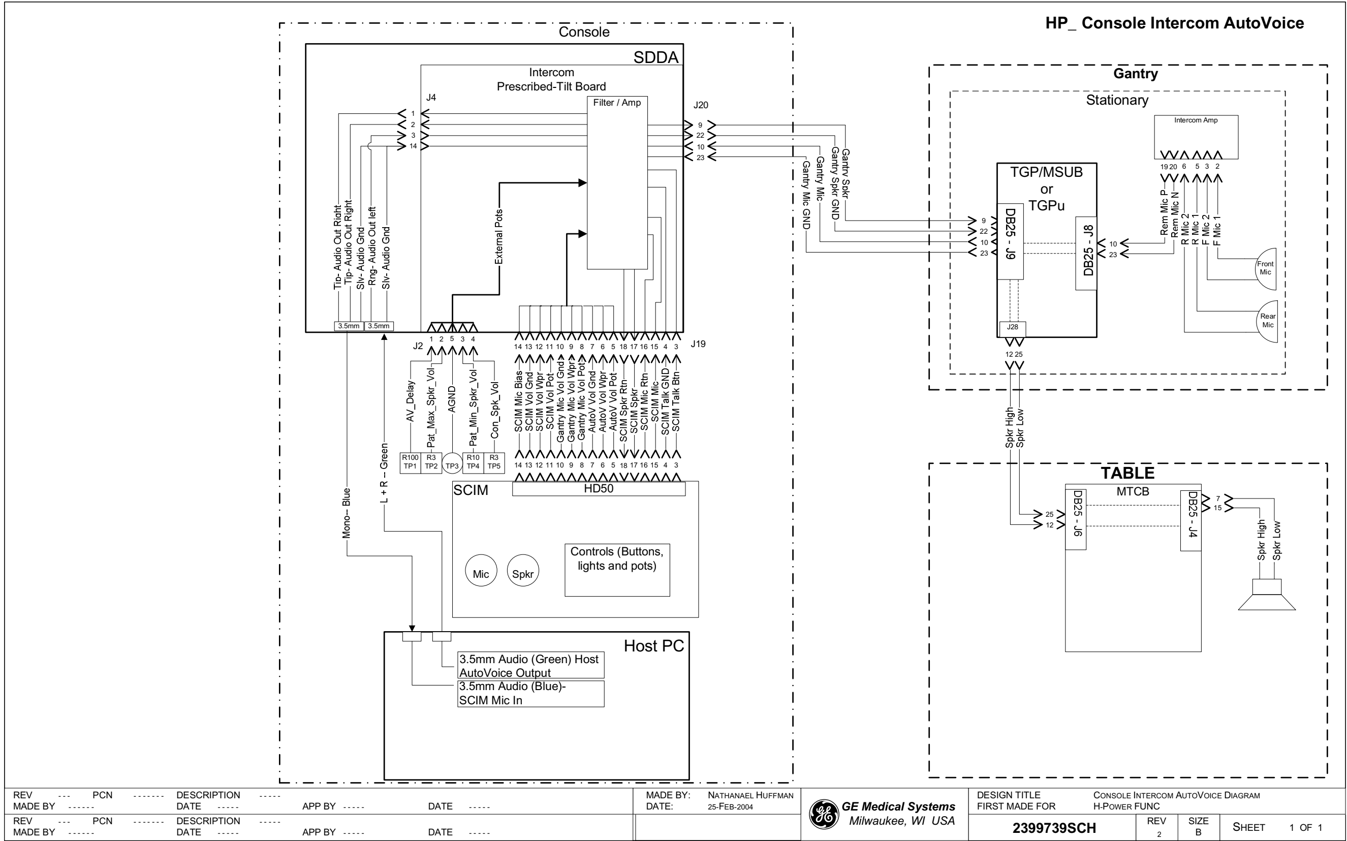
Figure 6-7 2399739 Sheet 1, Rev. 2
