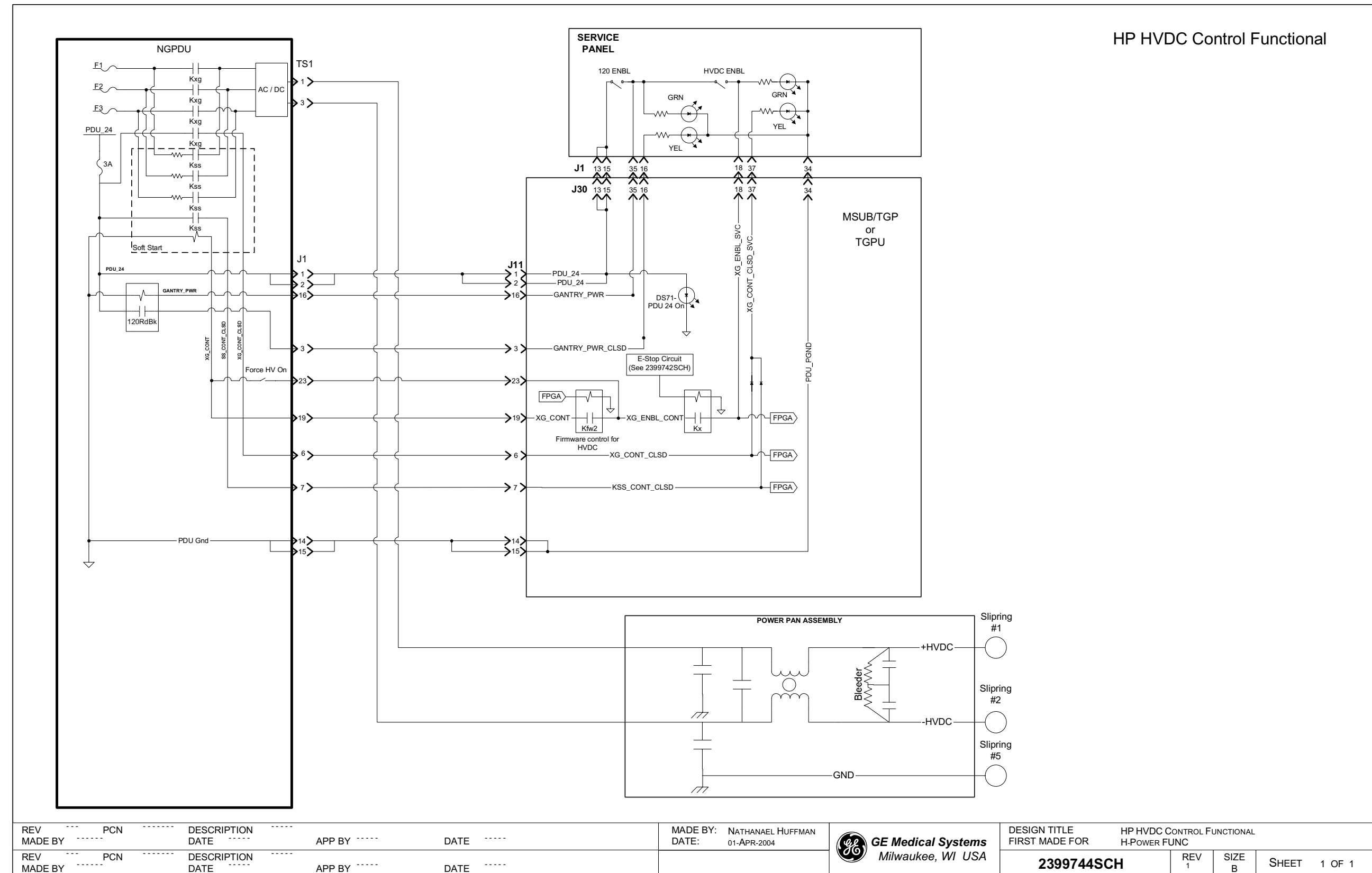
Figure 8-3 2399744 Sheet 1, Rev. 1
