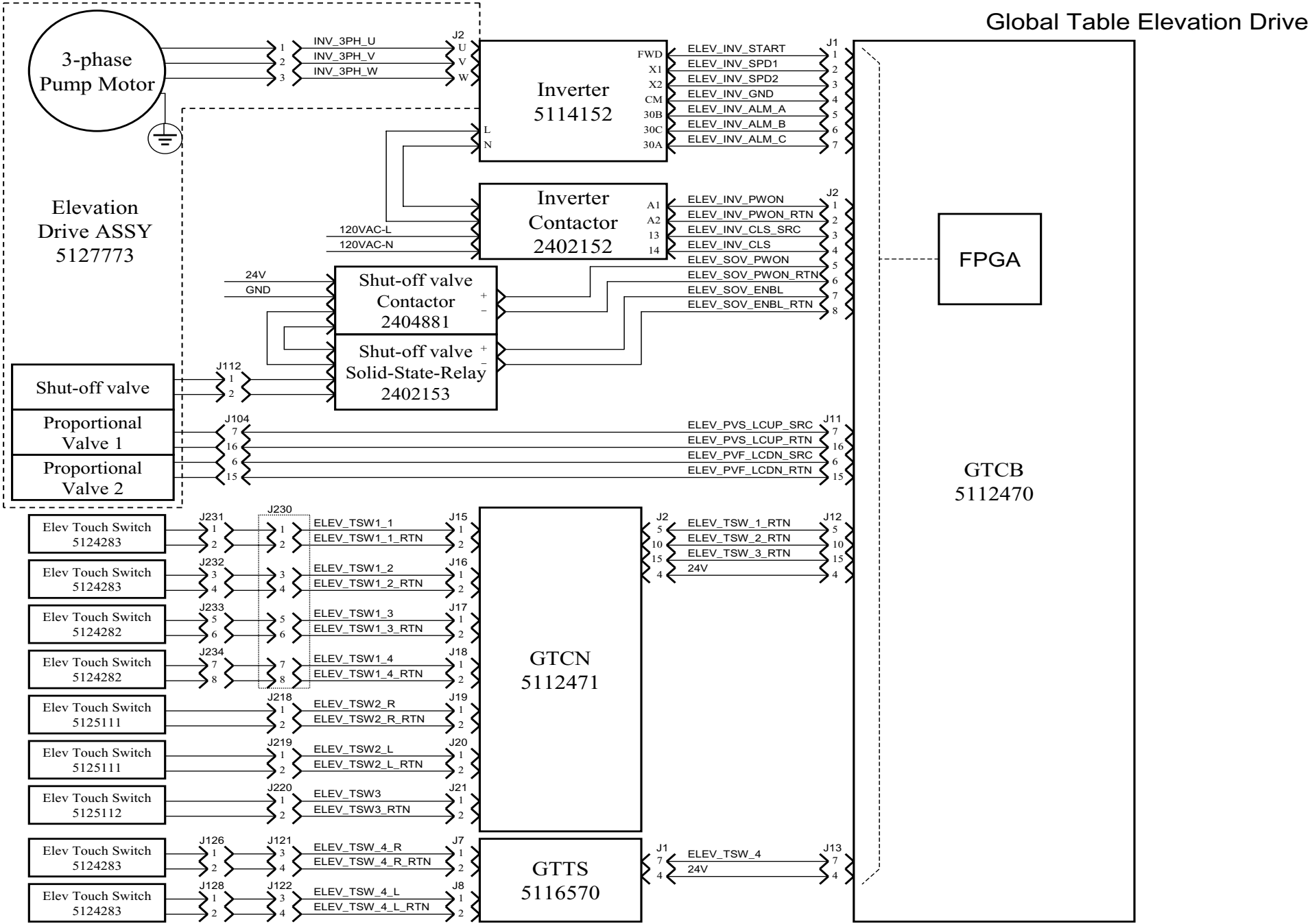
Figure 4-6 5127766 Sheet 3, Rev. 1
