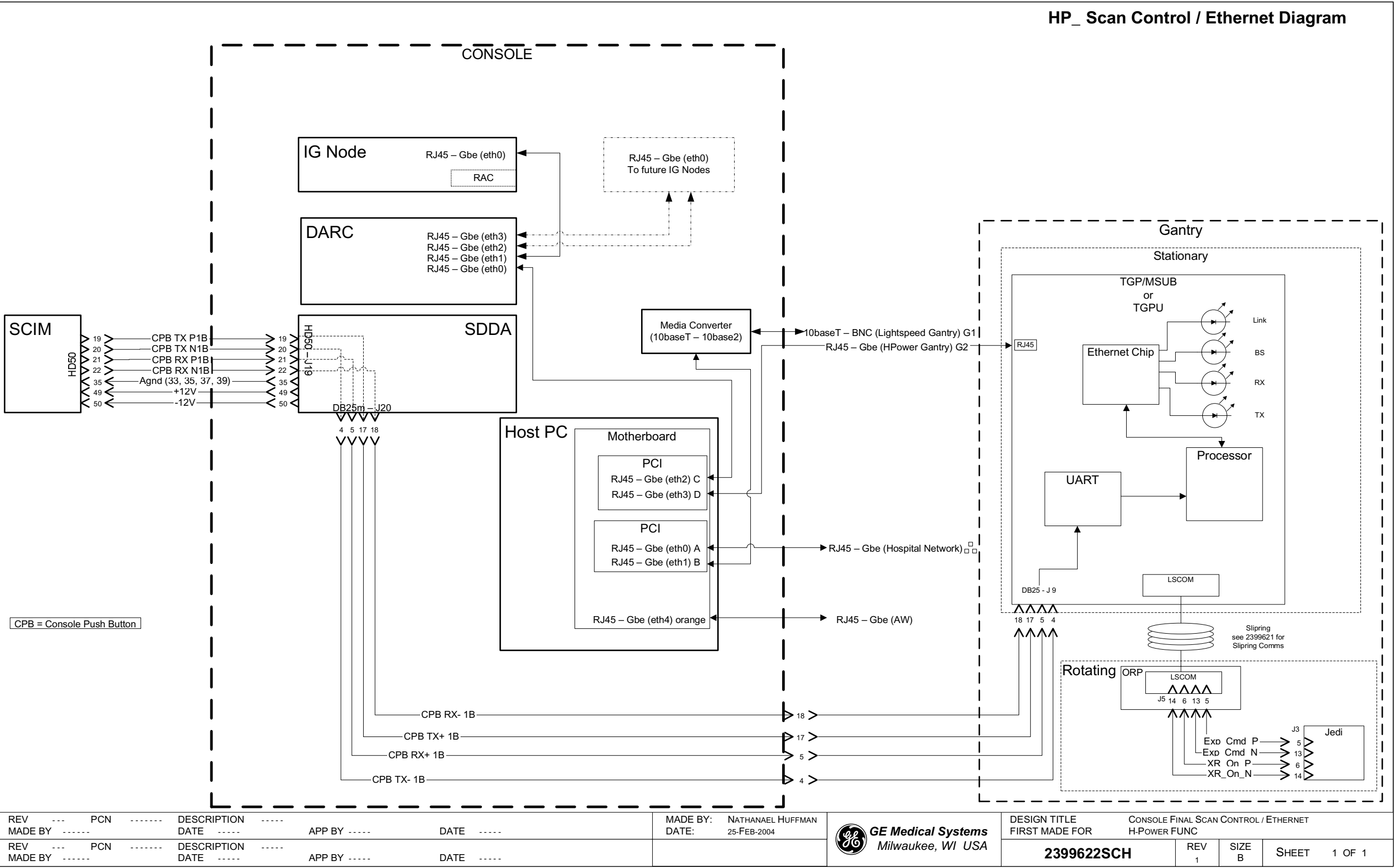
Figure 1-2 2399622 Sheet 1, Rev 1
