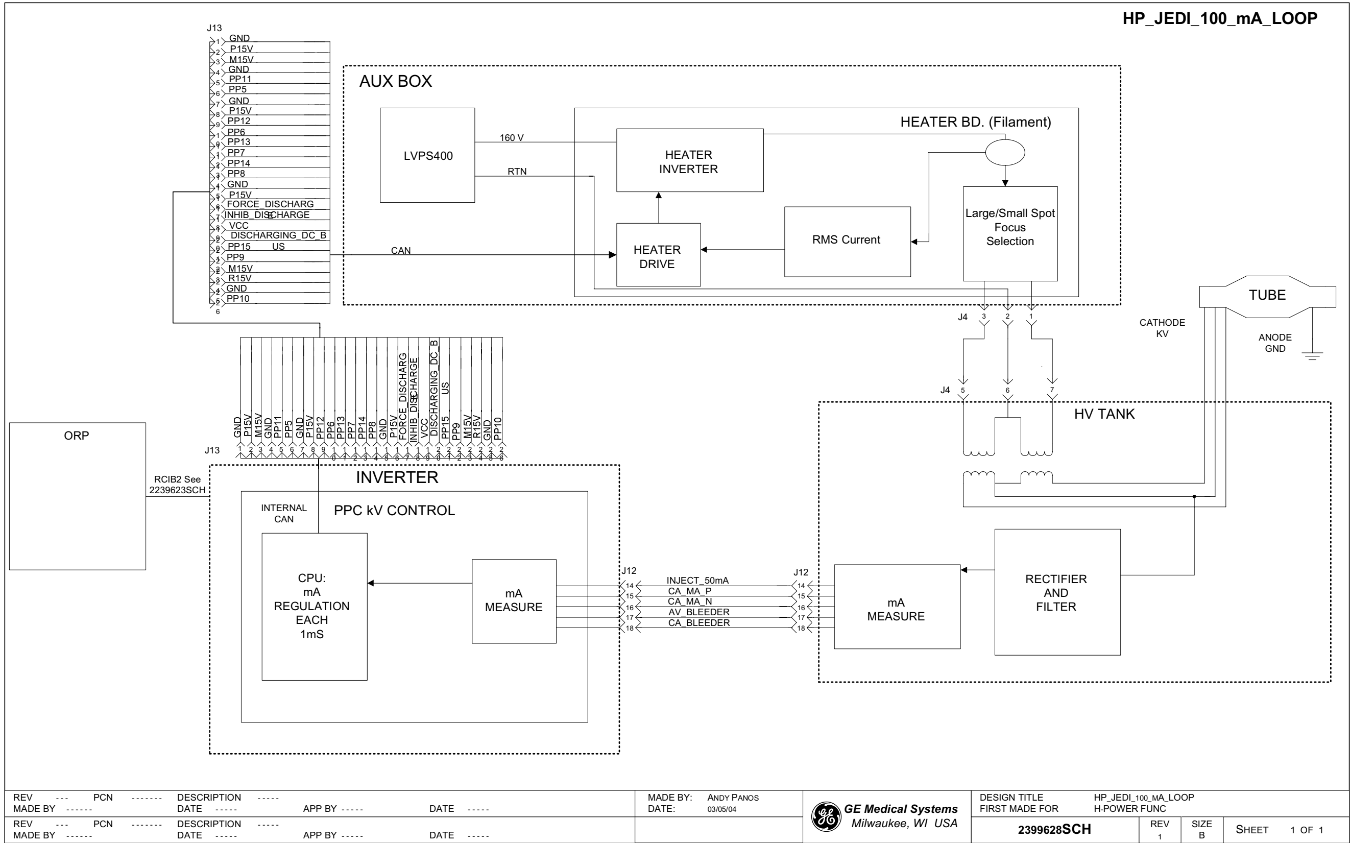
Figure 2-3 2399628 Sheet 1, Rev. 1
