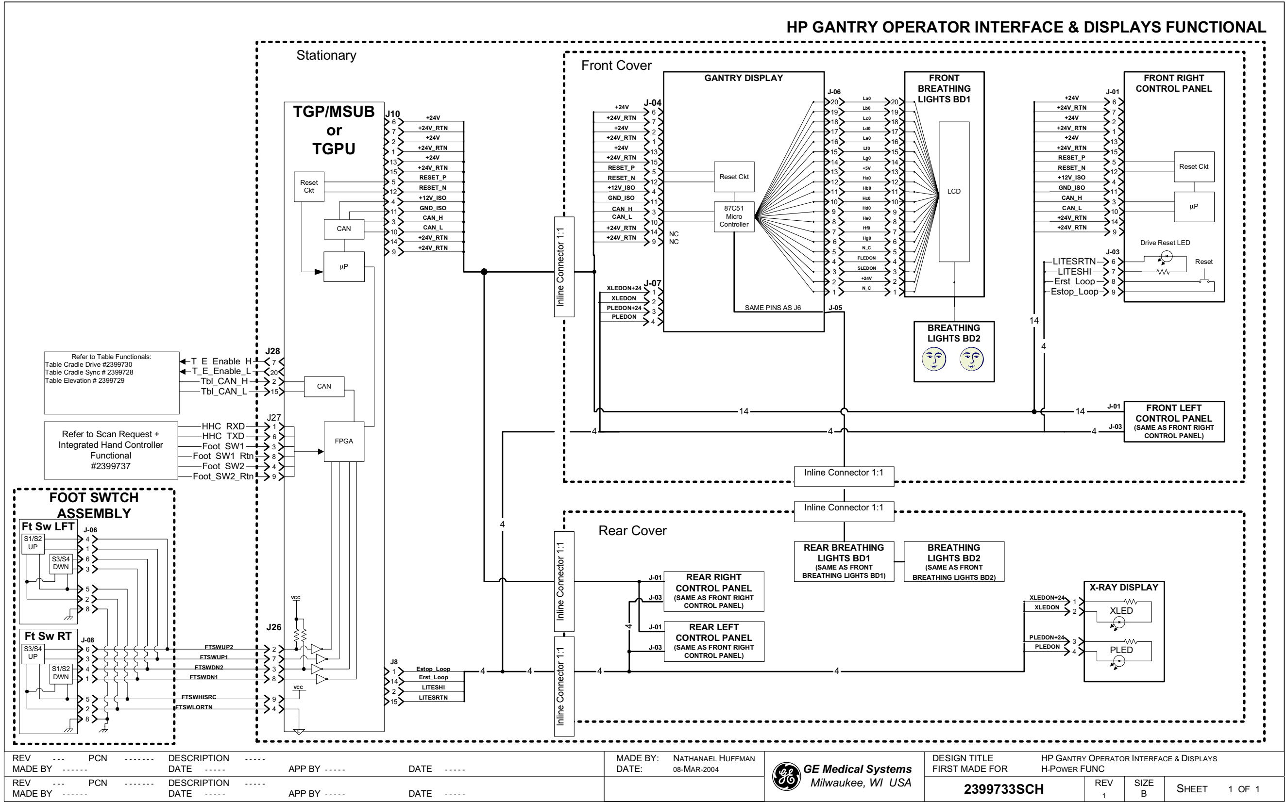
Figure 6-1 2399733 Sheet 1, Rev. 1
