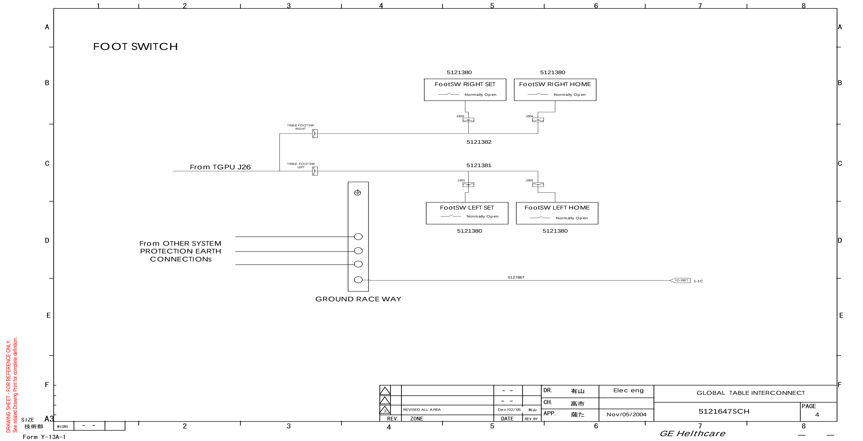
Figure 4-9 5121647 Sheet 4, Rev 3
