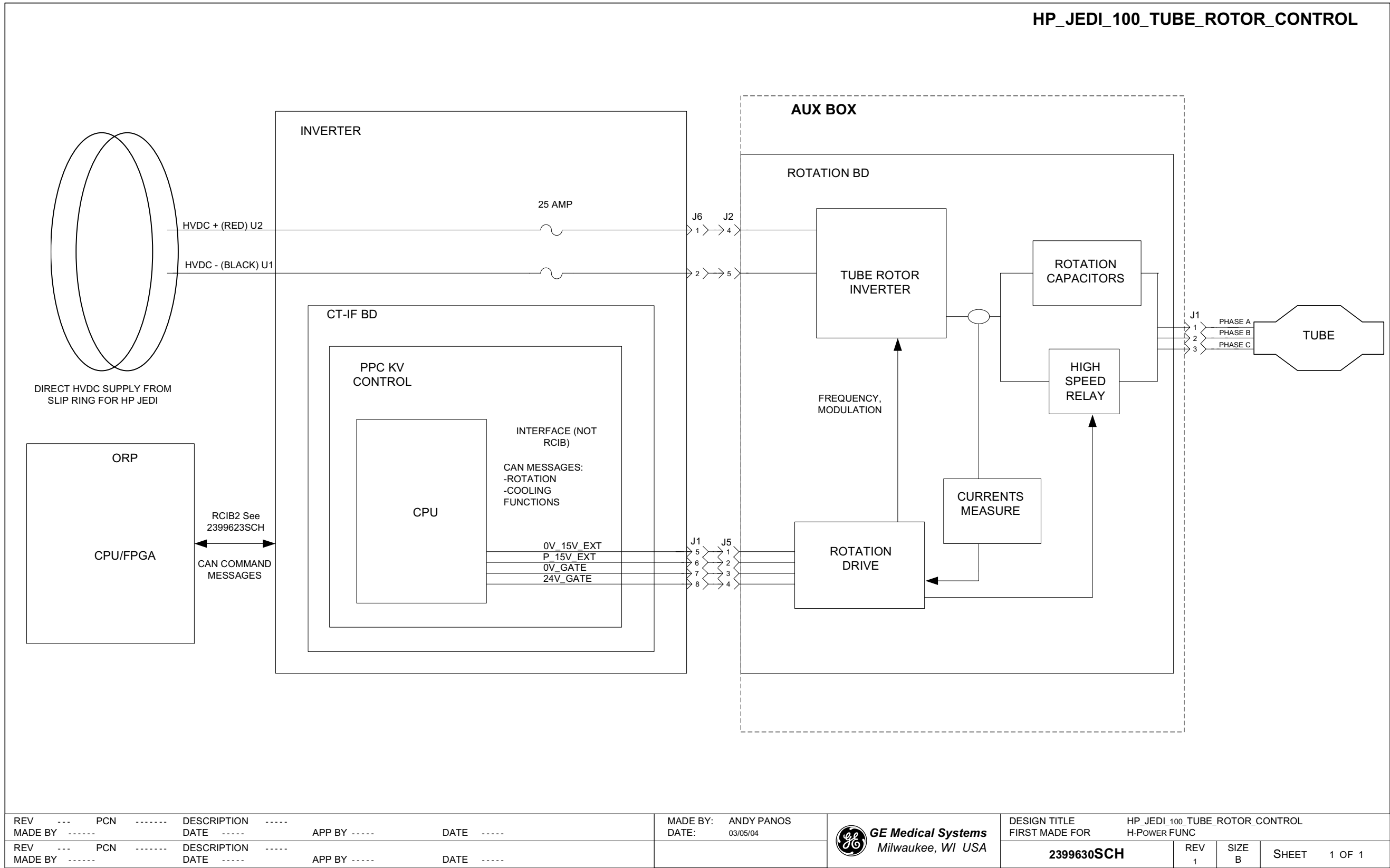
Figure 2-6 2399630 Sheet 1, Rev. 1
